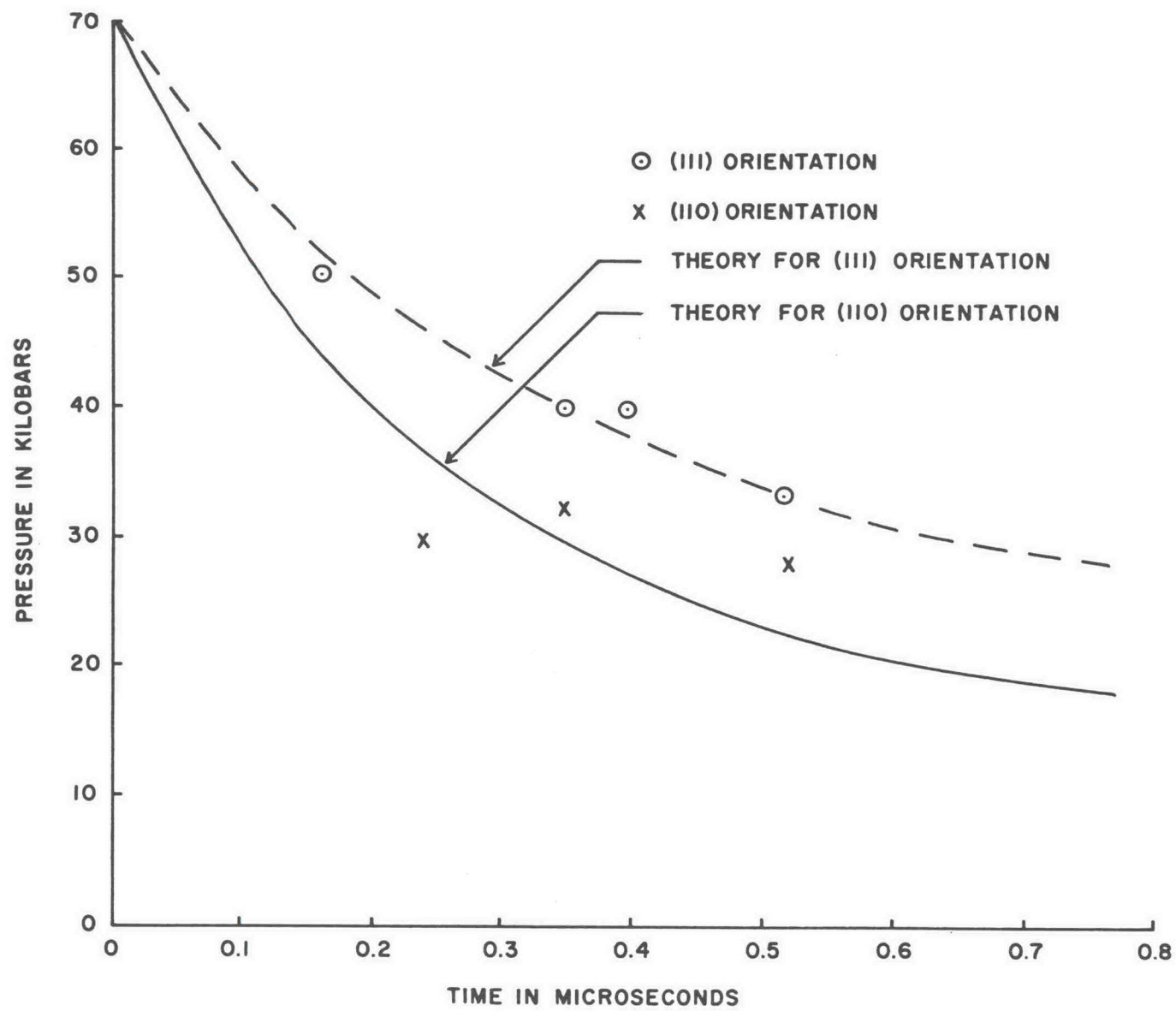
Fig. 29. Decay of elastic precursor wave in tungsten crystals shocked in [111] and [110] direction.
